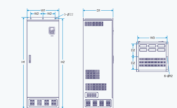
350-500kW Floor mounting Installation diagram
