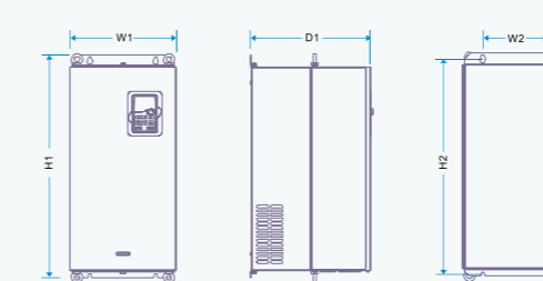
132-200kW Flange mounting Installation diagram
